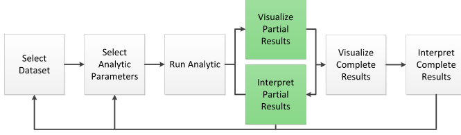
Fig. 2. A comparison between a traditional batch workflow and a workflow utilizing progressive visual analytics. The latter workflow avoids inefficiencies associated with ‘compute-wait-visualize’.
